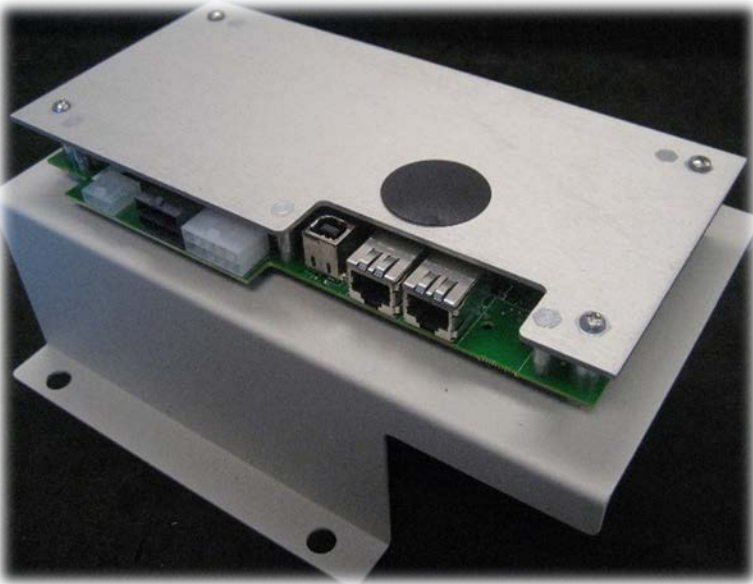
SFT populated PCB
